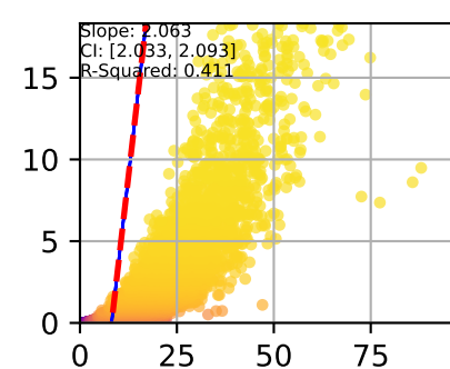
(Stochastic Binarization)
